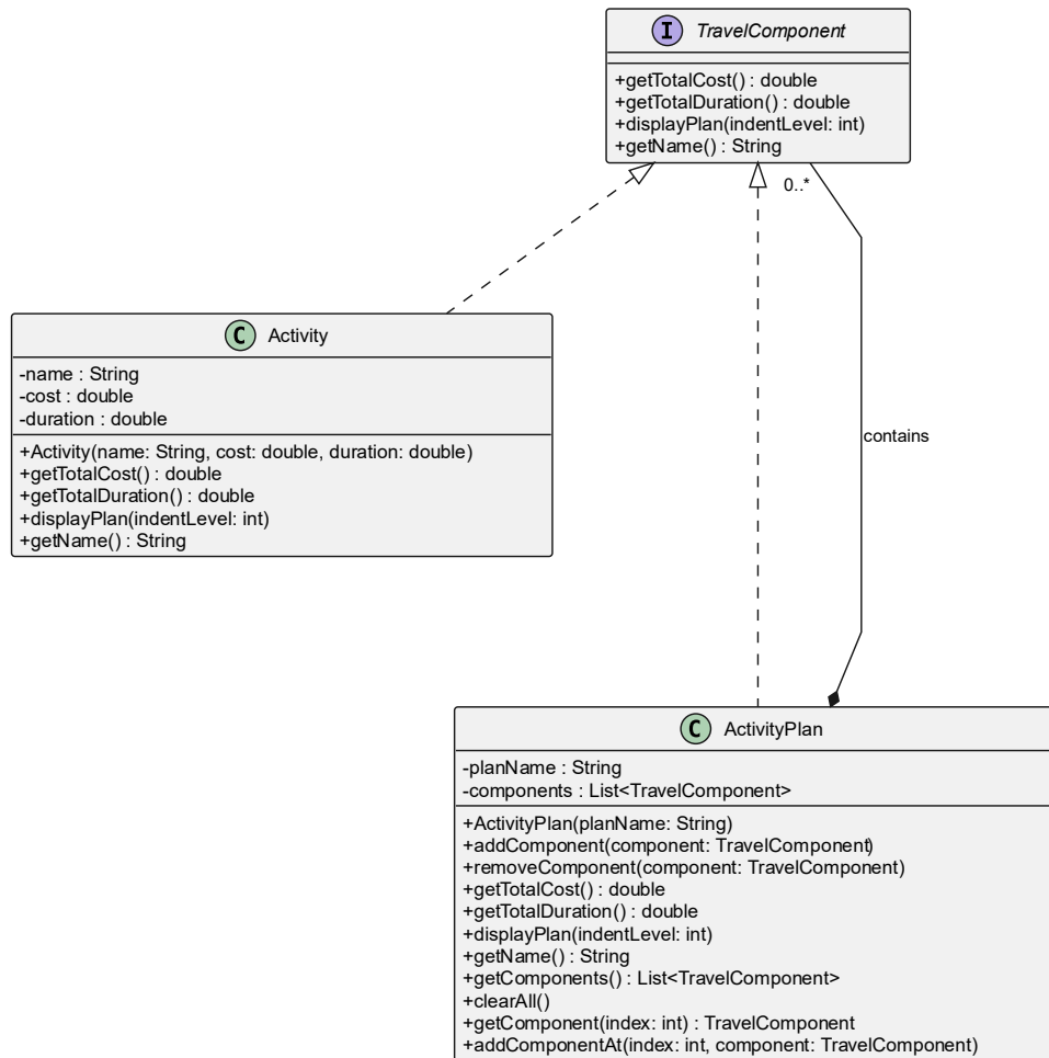
Smart Travel - Composite Design Pattern UML
