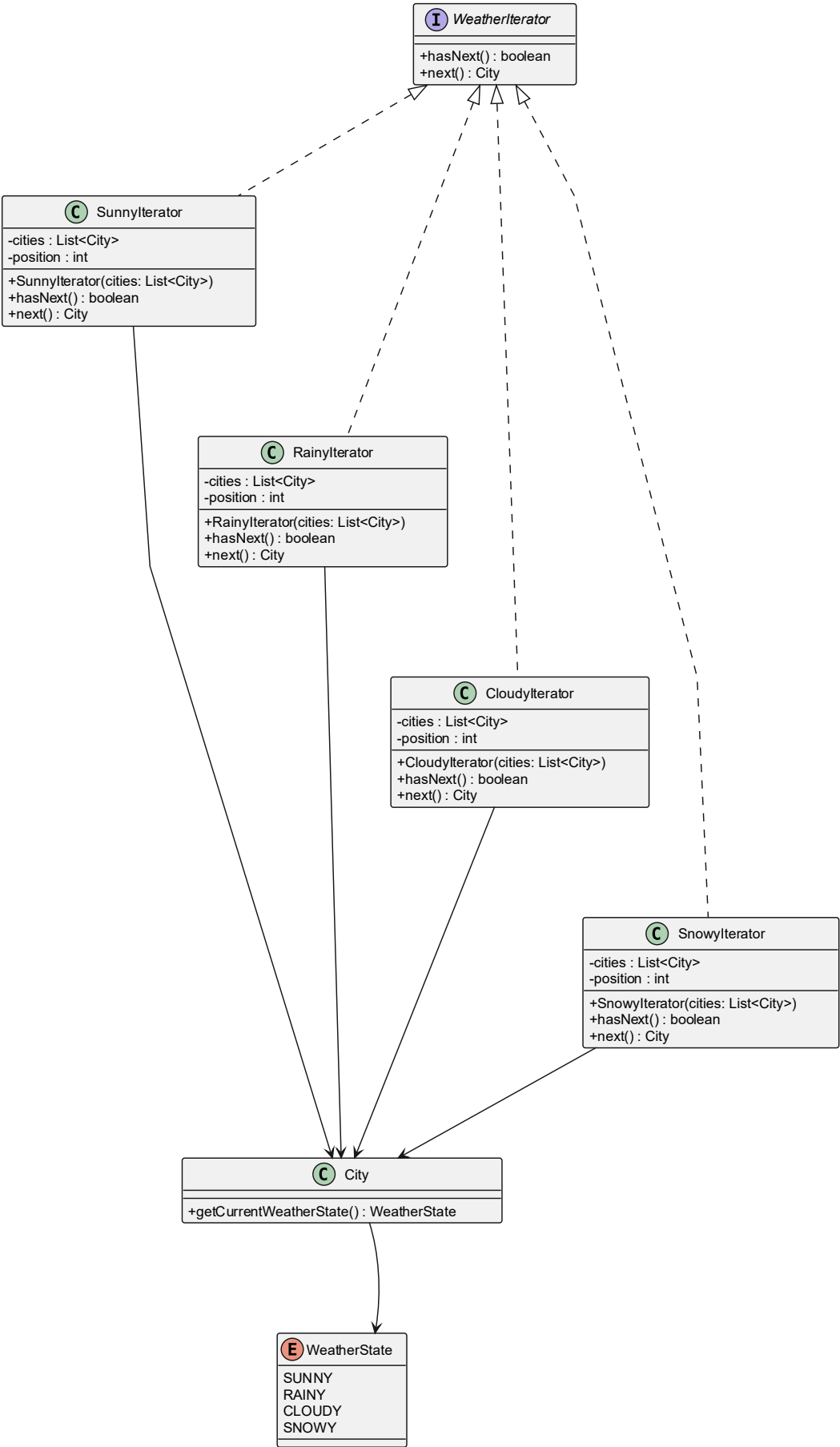
Smart Travel - Iterator Design Pattern UML
