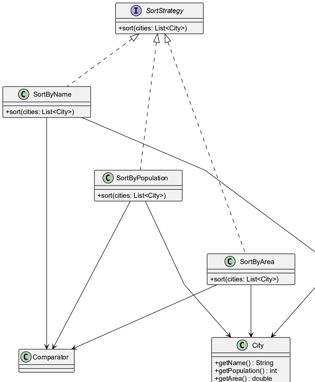
Smart Travel - Strategy Design Pattern UML
