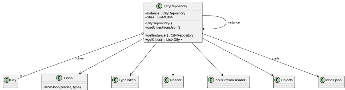
Smart Travel - Repository (Singleton) Design Pattern UML
